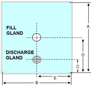
1000 Ltr - 2" Fill x 2" Cutter Membrane Discharge LLDPE 60mu Comprises of MET0000261 2" Gland Assembly - FILL MET0000262 2" Discharge Gland Assembly (with membrane).
